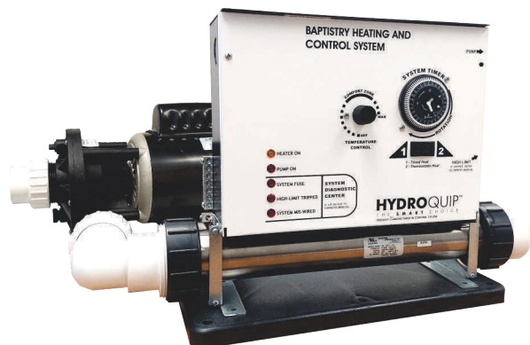
BES6000 (5.5kW) Series Shown
